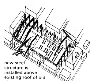
⑥ Installation of new steel structure begins
